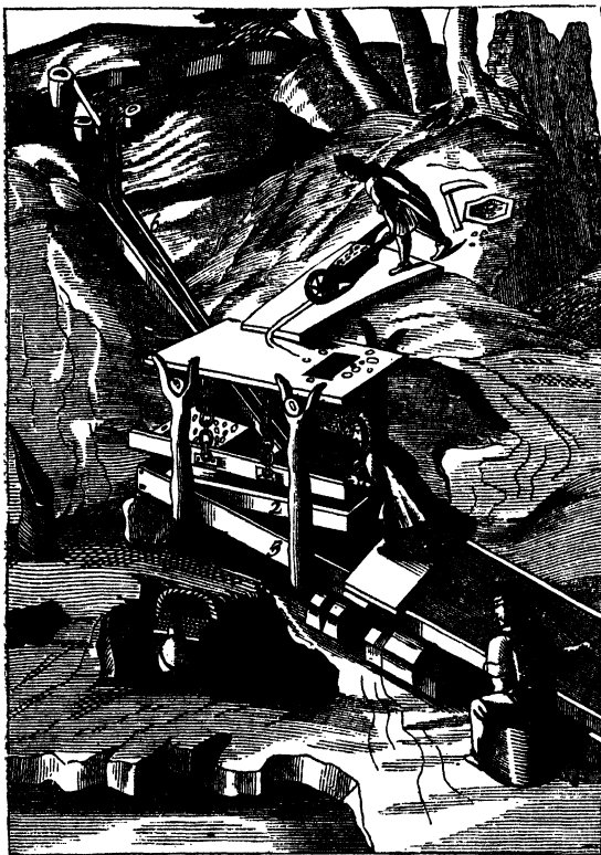
Fig. 105. Ancient Gold Washers (Pettus). "1. The man that worketh with the Battar (or shaking sieve). 2. The middle floor, whereon that which goeth through the Battar doth fall. 3. The lower floor, whereon that which cometh from the middle floor doth fall. 4. The plain receiver, called the hearth, of that which falls from both. 5. The person that stands on a board, and out of a wheelbarrow throws the matter or oar into the tunnel which guides it into the Battar. 6. The channel in which water doth run into the Battar."
